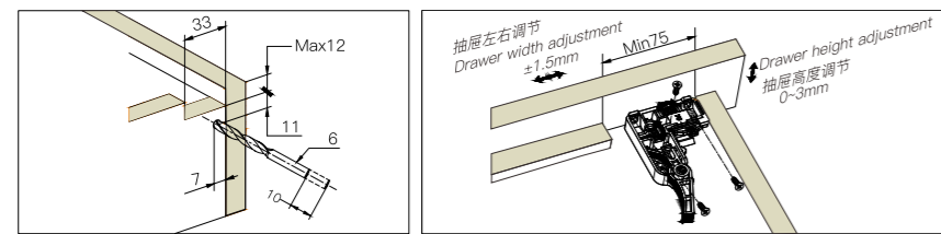
抽屉尺寸和钻孔(mm) Drawer size and drilling
